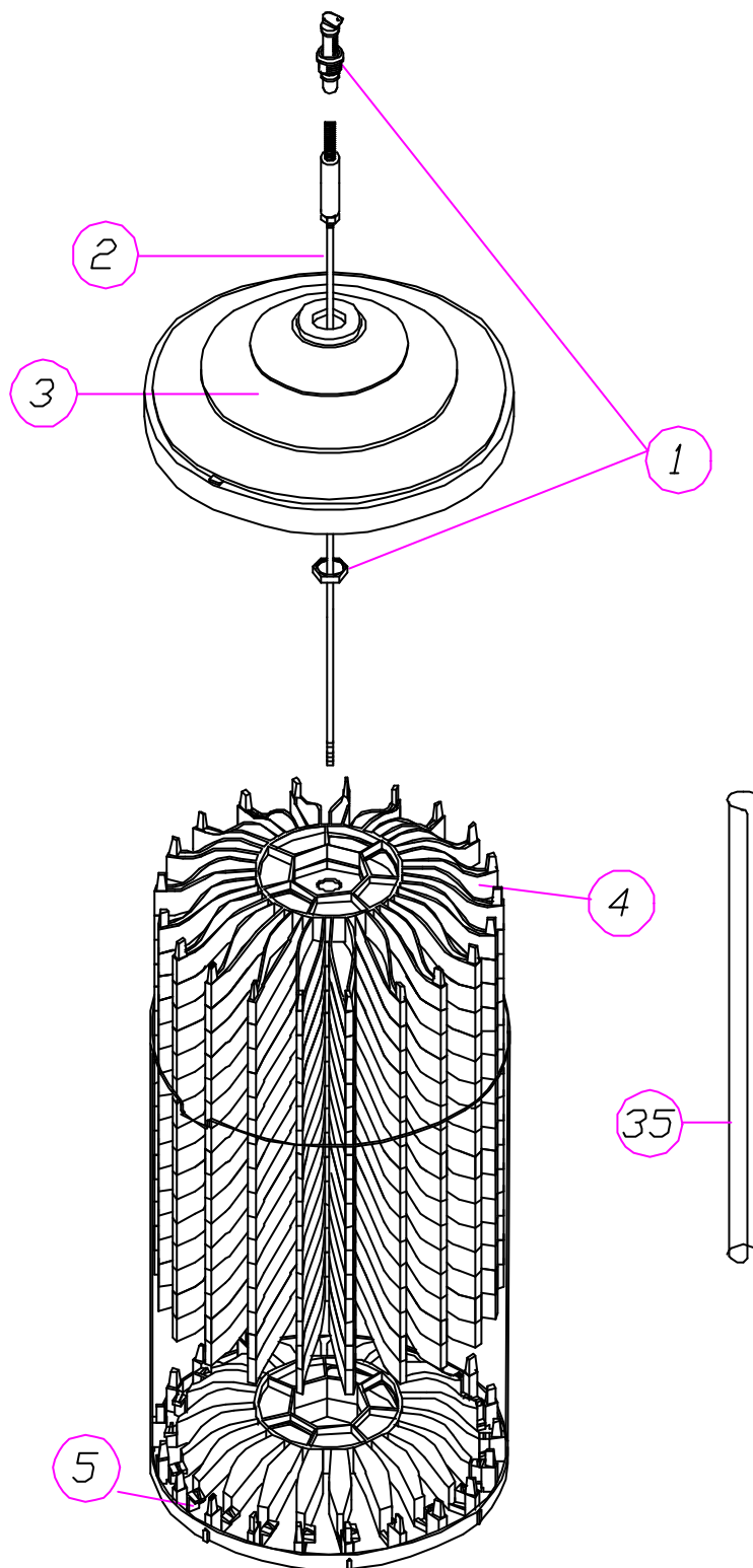
PICTURE 2 PARTS
