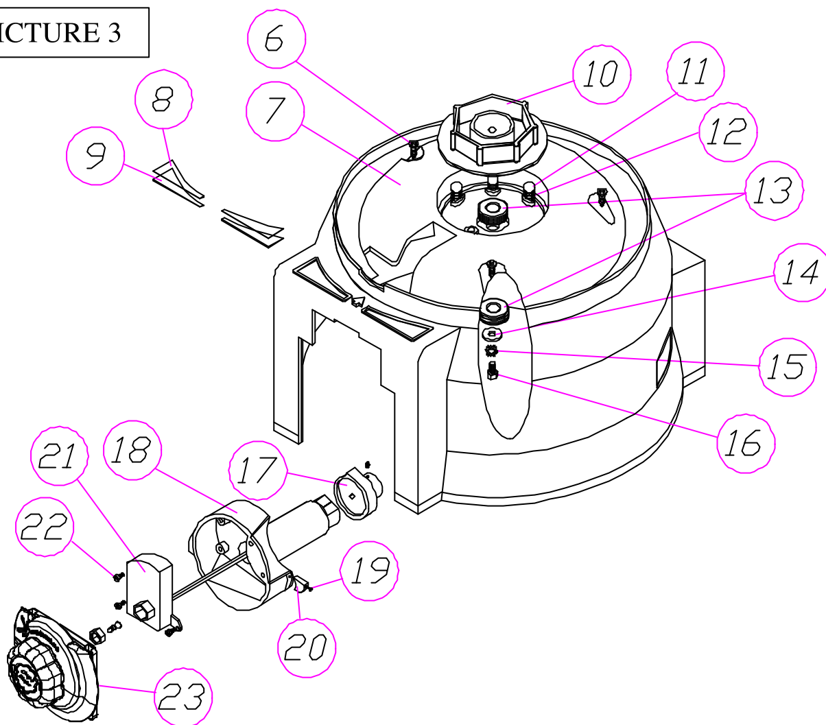
PICTURE 3 PARTS
